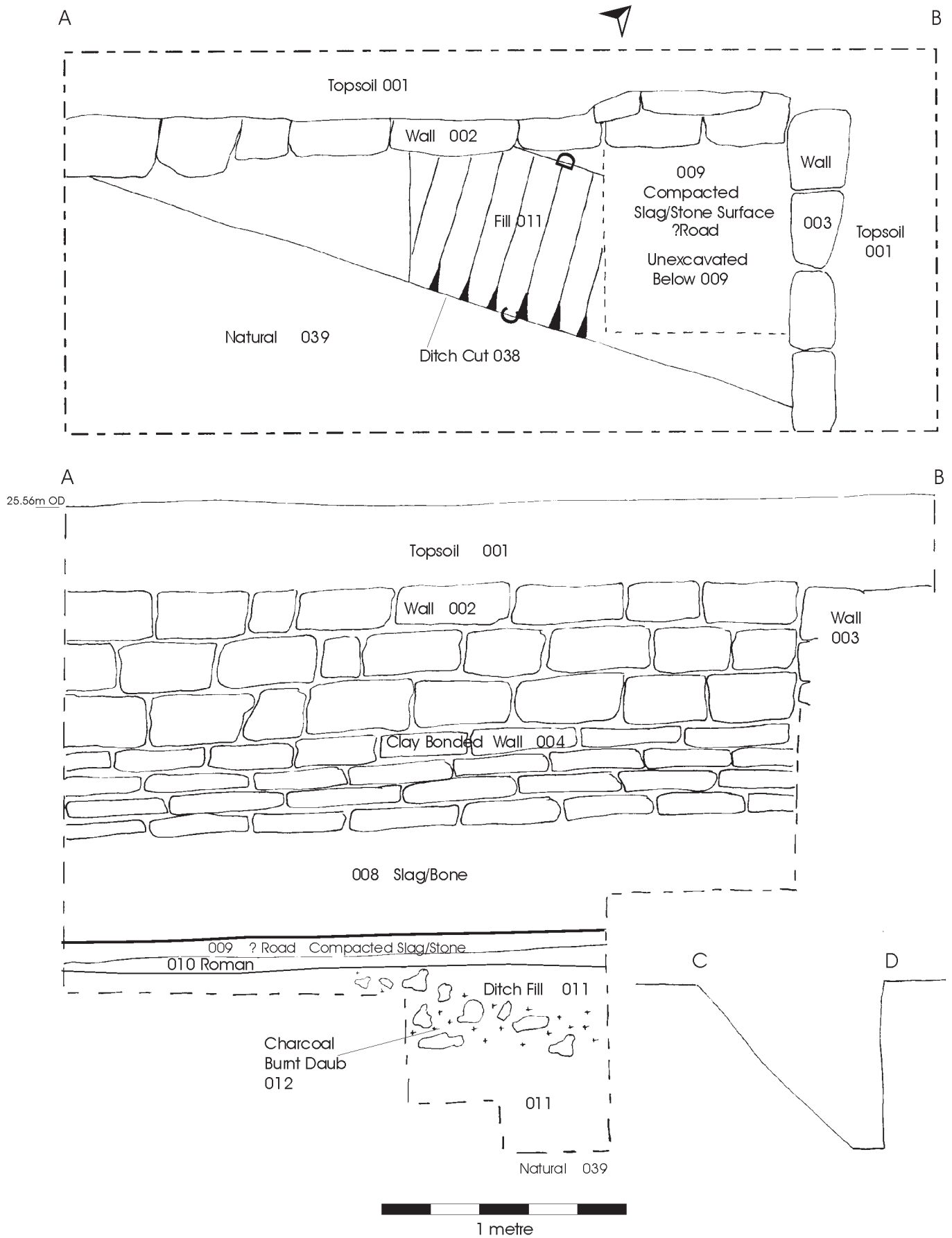
Fig. 8 The Barton, Monmouth : Trench A : Section A-B and Ditch Profile C-D
